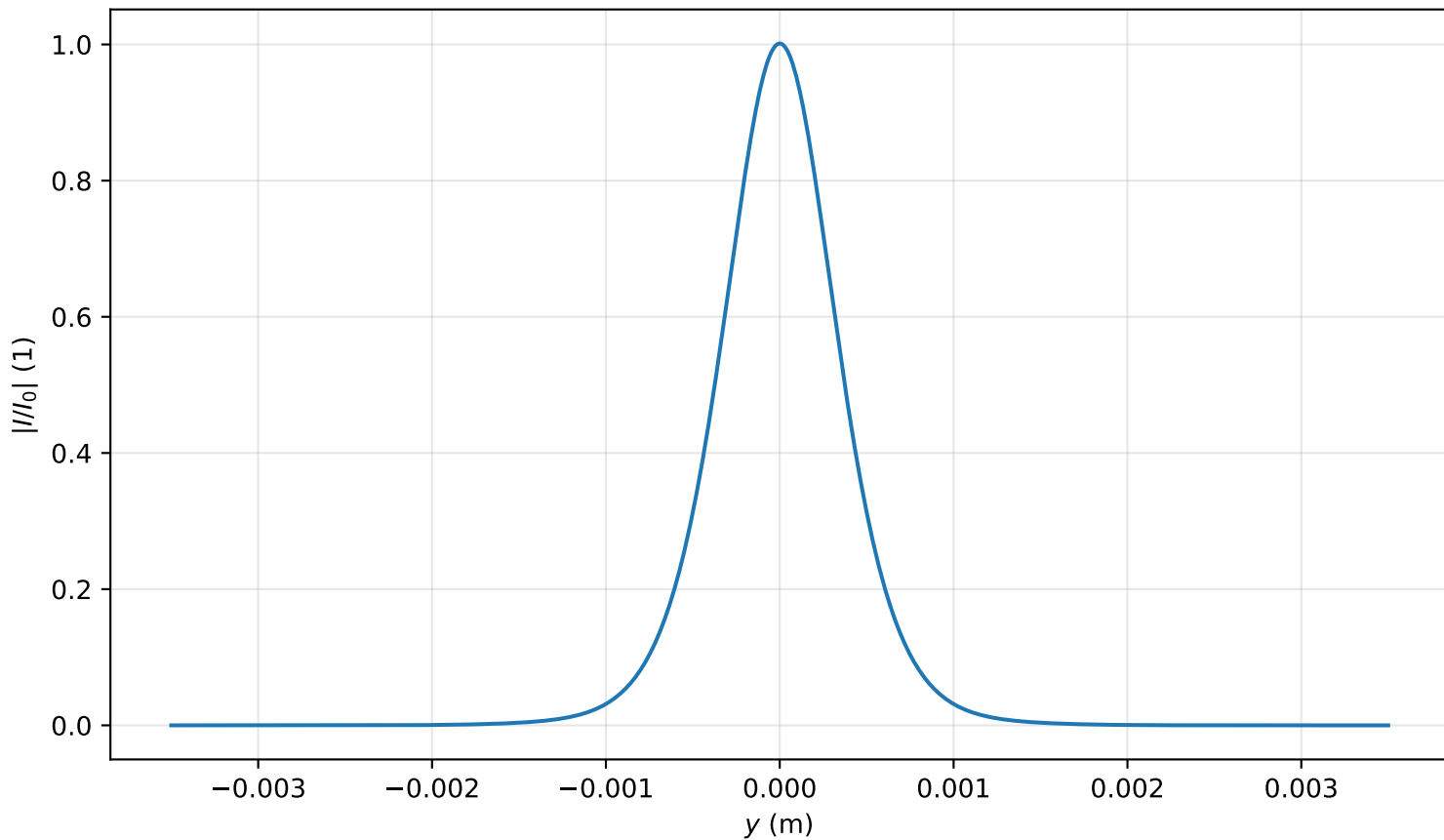
Intensity profile I(x=0, y, z=2.388)/I_0 , P_{in}=0.7P_{cr} , artificial time
